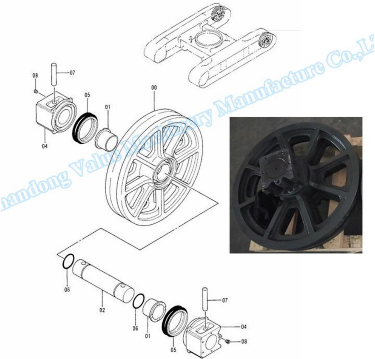
FRONT IDLER
